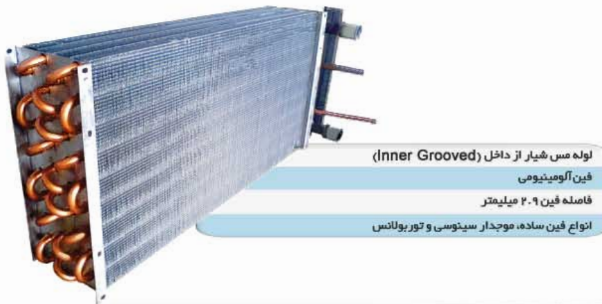
Inner Grooved Coil
